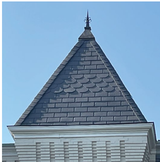
Figure 10a and 10b. Polymer slates offer a choice of shapes but not sizes, limiting their ability to achieve a good visual match for some historic slate. With the size of the polymer slates (Figure 11b) being nearly twice that of the historic slates (11a), the scale of the entire feature is incompatibly altered. The molded edges of this material, which contribute to its ability to replicate slate, would be lost if each shingle was resized by cutting. Photo: John Sandor, NPS.
