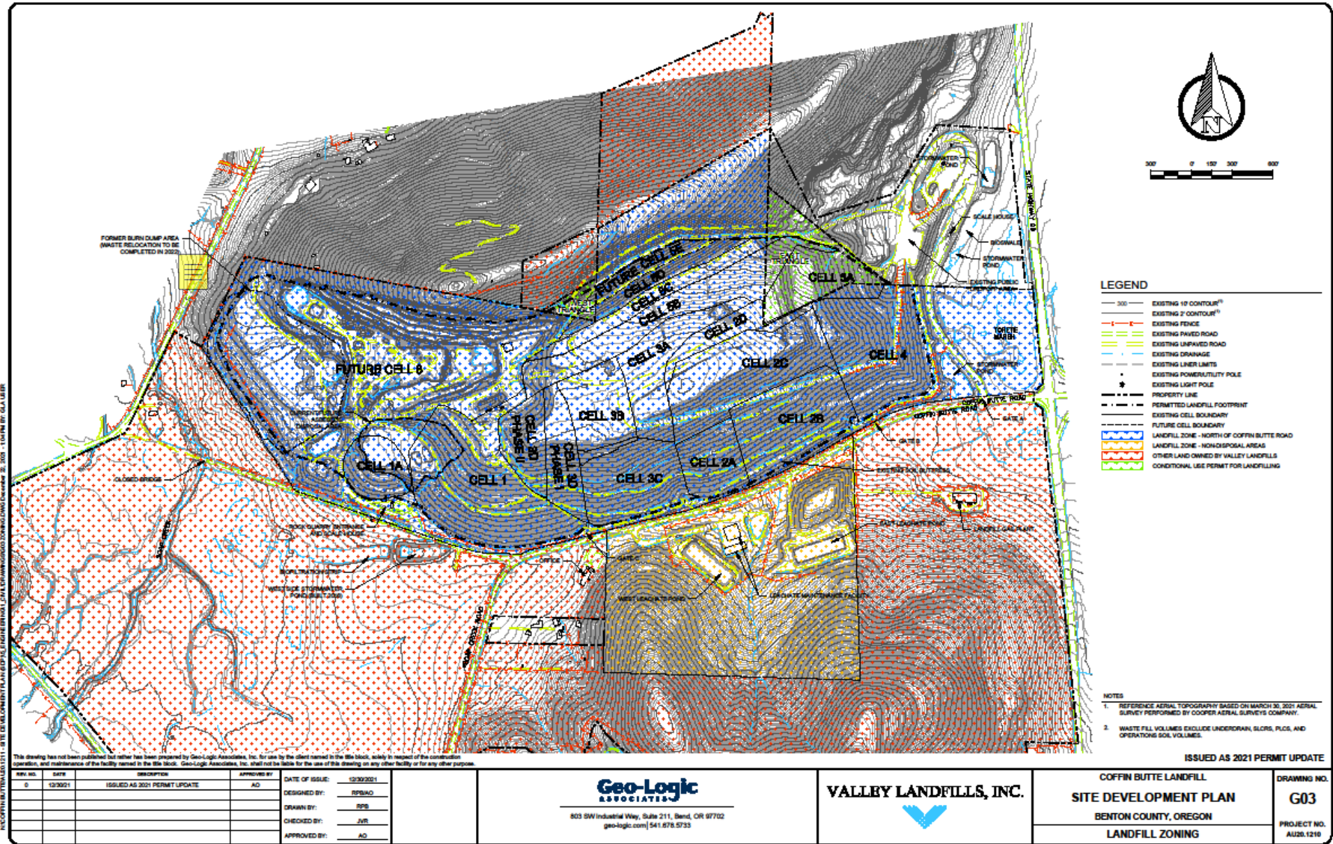
Figure 12: Landfill Zoning
